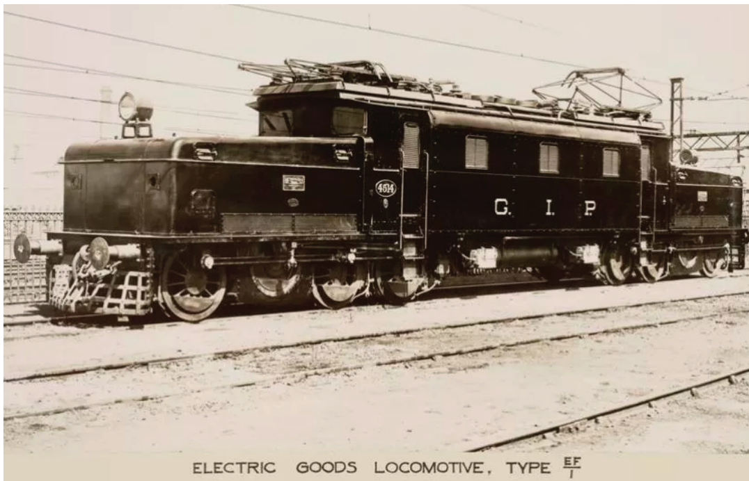
ELECTRIC LOCOMOTIVE TYPE EF 1, NUMBER 4514. THIS BROAD GAUGE (5'6") LOCOMOTIVE RAN ON THE GREAT INDIAN PENINSULA
